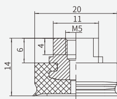
Suction cup 4×20 5×20 6×20 8×20
