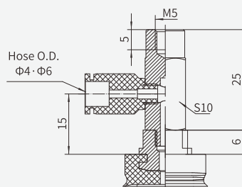
Suction cup 4×20 5×20 6×20 8×20
