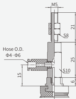
Suction cup 4×20 5×20 6×20 8×20
